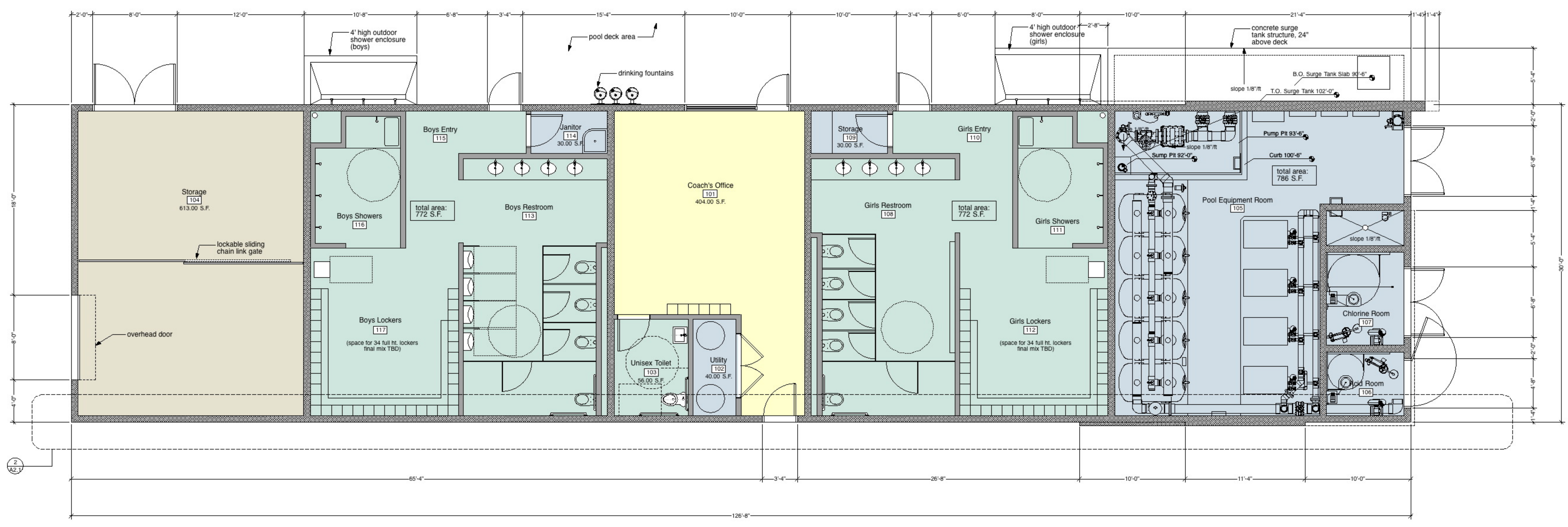
First Floor Plan 1
